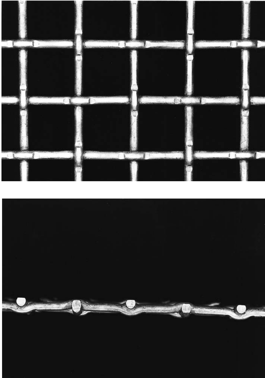
FIG. 4 Lock Crimp
